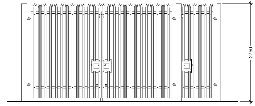
TYPICAL 3-POINT PALISADE FENCE AND GATES 1:50 @ A1
